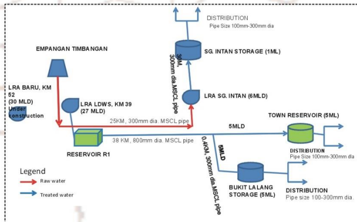
Preliminary Water Reticulation System Schematic
